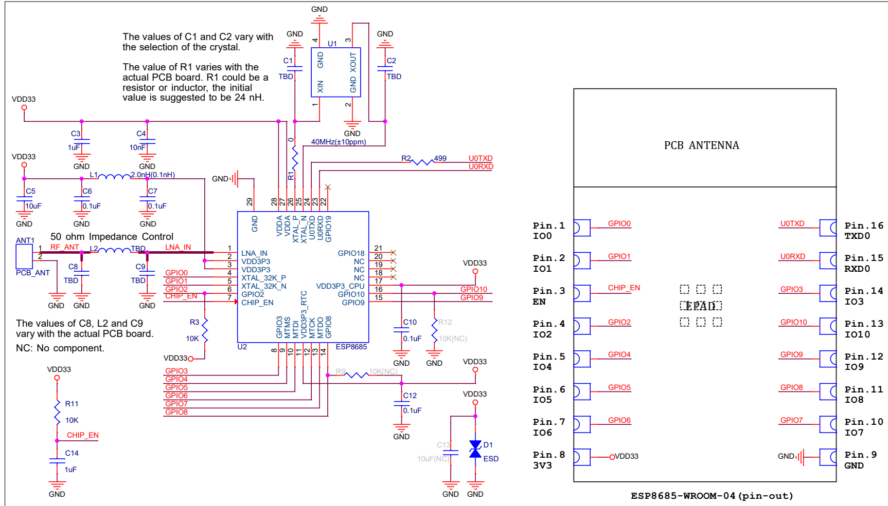
Figure 8-1. Schematics
