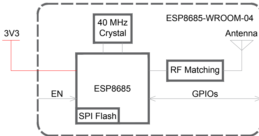
Figure 2-1. Block Diagram
