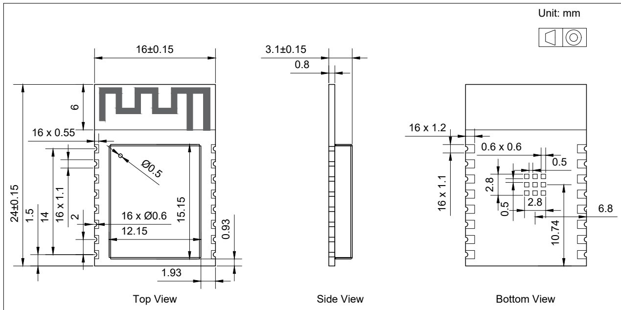
Figure 10-1. Physical Dimensions
