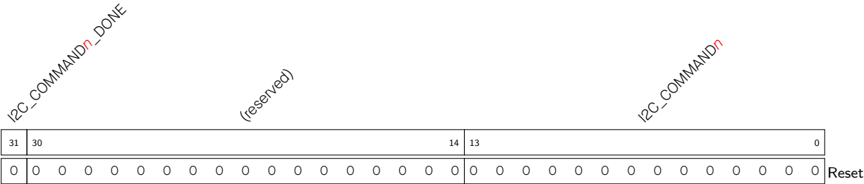
Register 21.21. I2C_COMD n _REG ( n : 0-15) (0x58+4* n )
