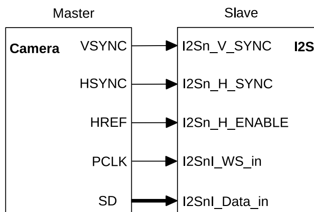
Figure 22.5-4. Camera Slave Receiving Mode
