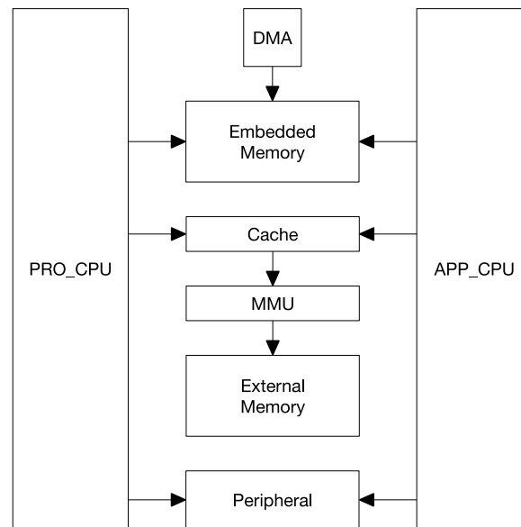
Figure 3.2-1. System Structure
