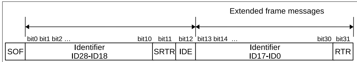
Figure 25.5-5. Positions of Arbitration Lost Bits
