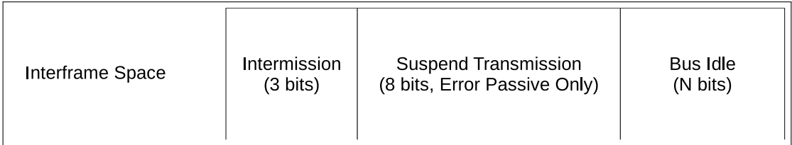
Figure 25.3-4. The Fields within an Interframe Space
