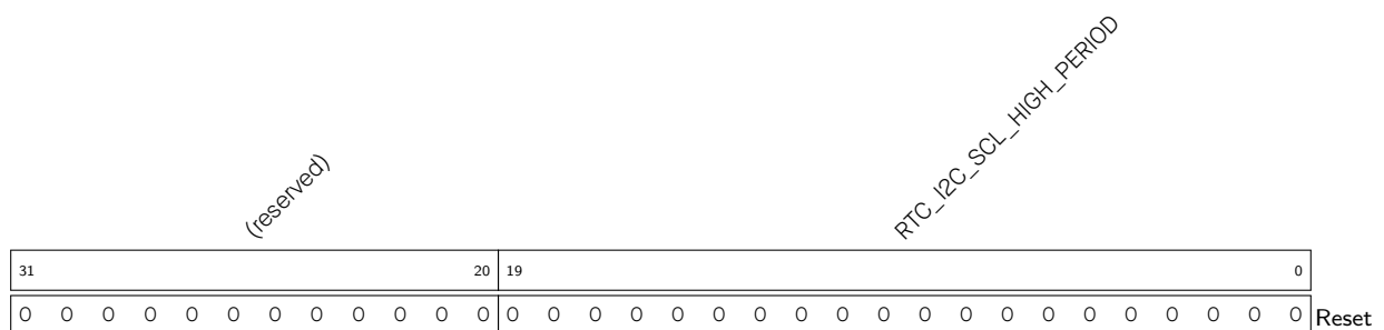
Register 1.17. RTC_I2C_SCL_HIGH_PERIOD_REG (0x038)
