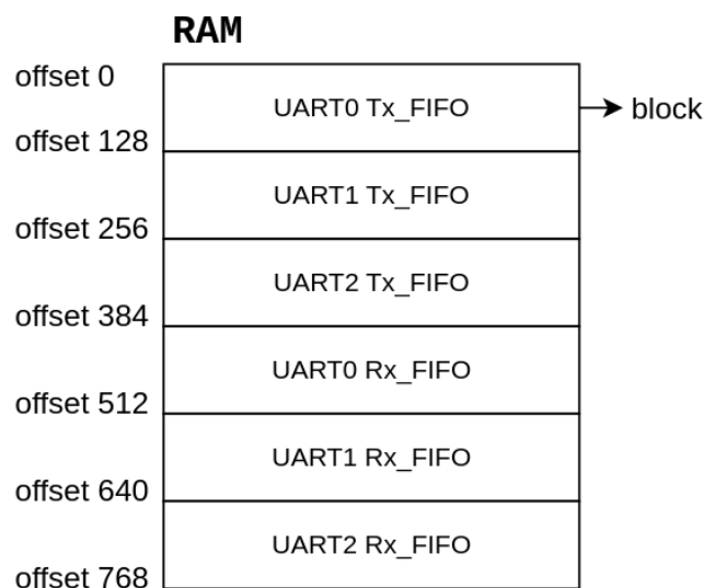
Figure 19.3-2. UART Shared RAM
