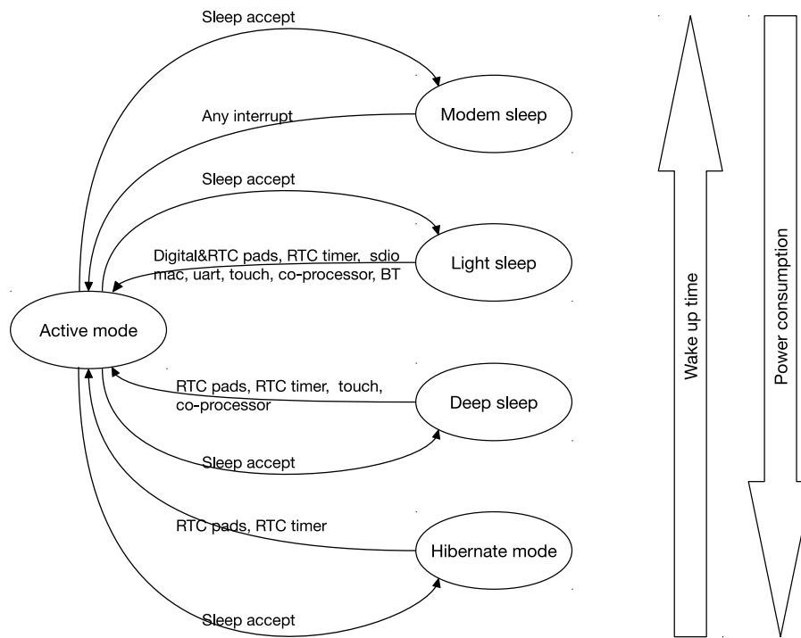
Figure 9.3-8. Power Modes
