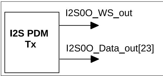
Figure 22.4-8. PDM Sends Signal
