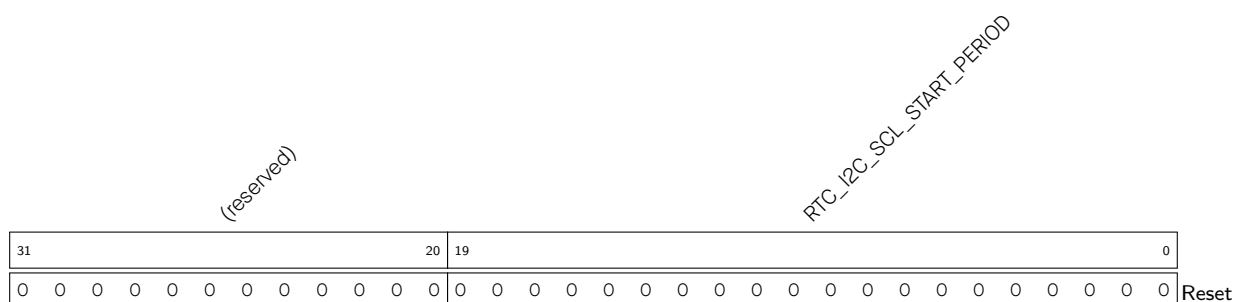
Register 1.18. RTC_I2C_SCL_START_PERIOD_REG (0x040)
