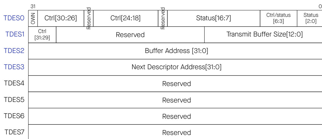
Figure 24.8-1. Transmit Descriptor
