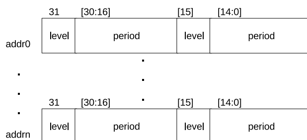
Figure 30.2-2. Data Structure
