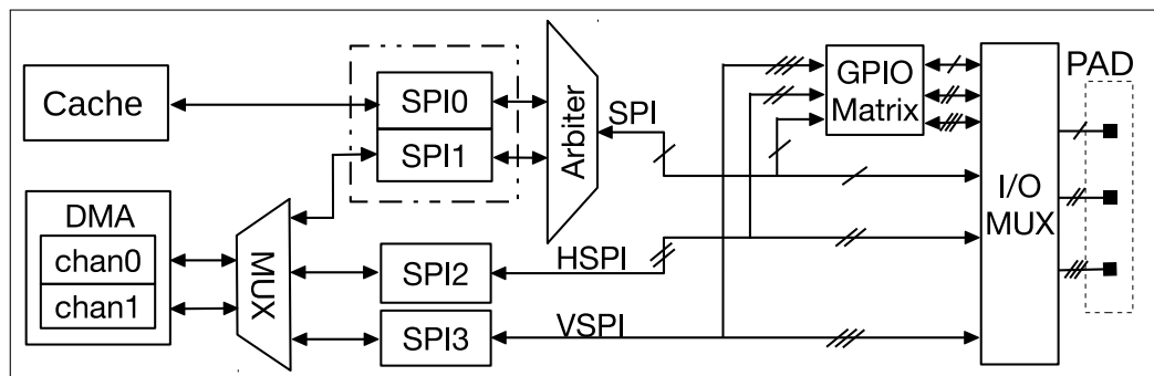
Figure 20.1-1. SPI Architecture
