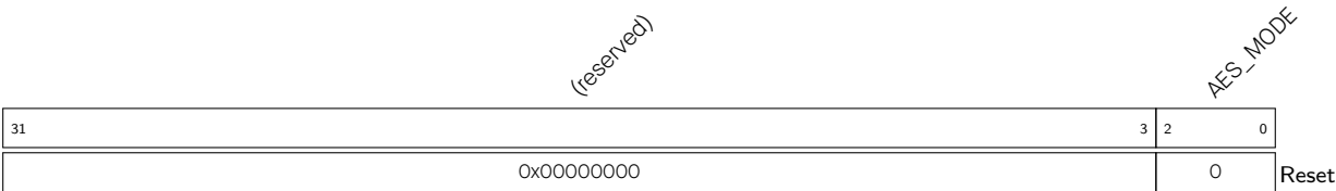
Register 14.3. AES_MODE_REG (0x008)
