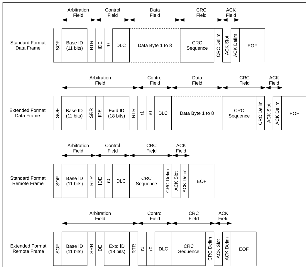
Figure 25.3-1. The bit fields of Data Frames and Remote Frames
