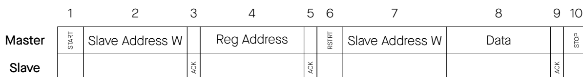
Figure 1.6-2. I2C Write Operation
