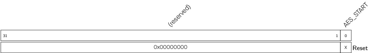
Register 14.1. AES_START_REG (0x000)
