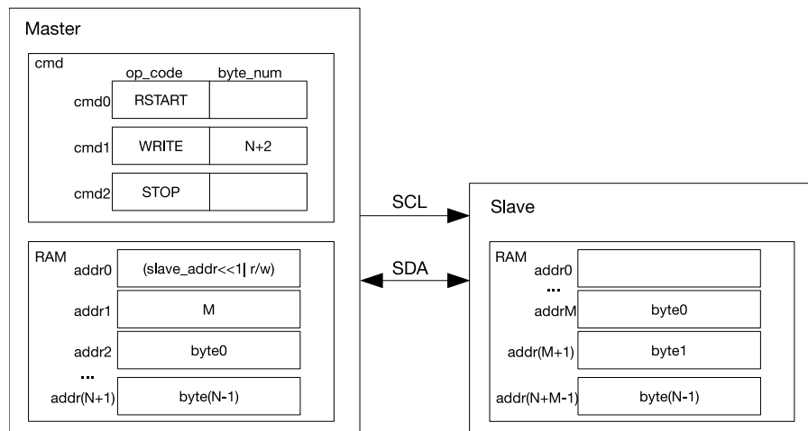
Figure 21.3-7. I2C Master Writes to addrM in RAM of Slave with 7-bit Address
