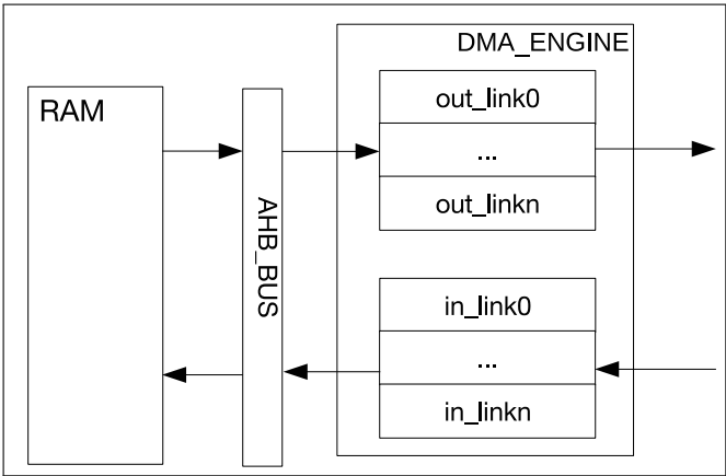
Figure 2.3-1. DMA Engine Architecture
