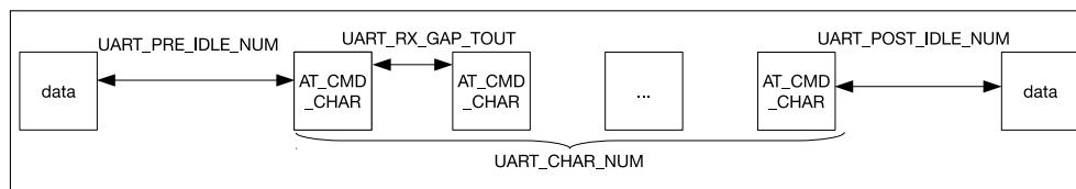
Figure 19.3-4. AT_CMD Character Format
