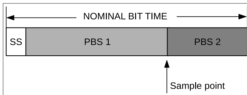
Figure 25.3-5. Layout of a Bit
