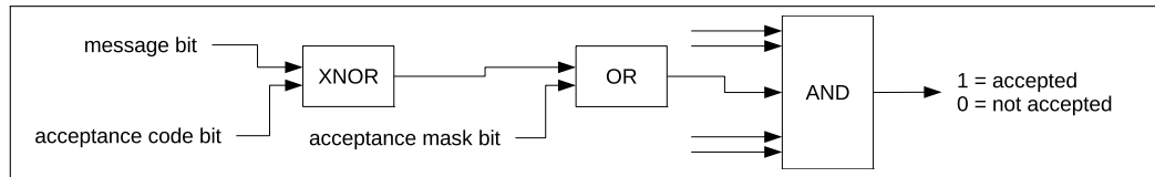
Figure 25.5-1. Acceptance Filter
