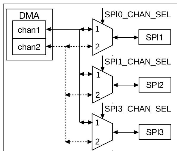
Figure 2.5-1. SPI DMA
