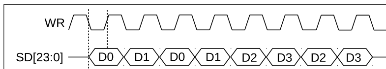
Figure 22.5-3. LCD Master Transmitting Data Frame, Form 2
