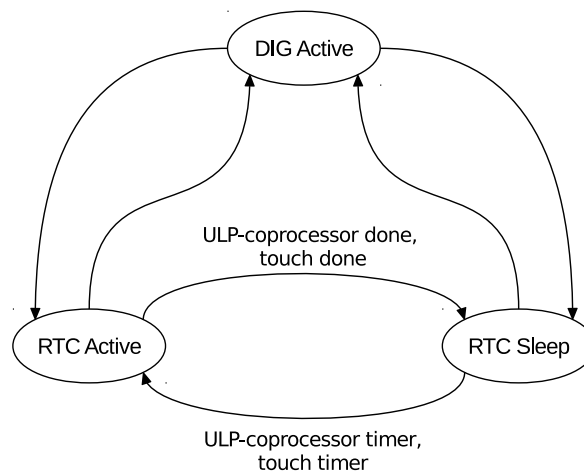
Figure 9.3-7. RTC States
