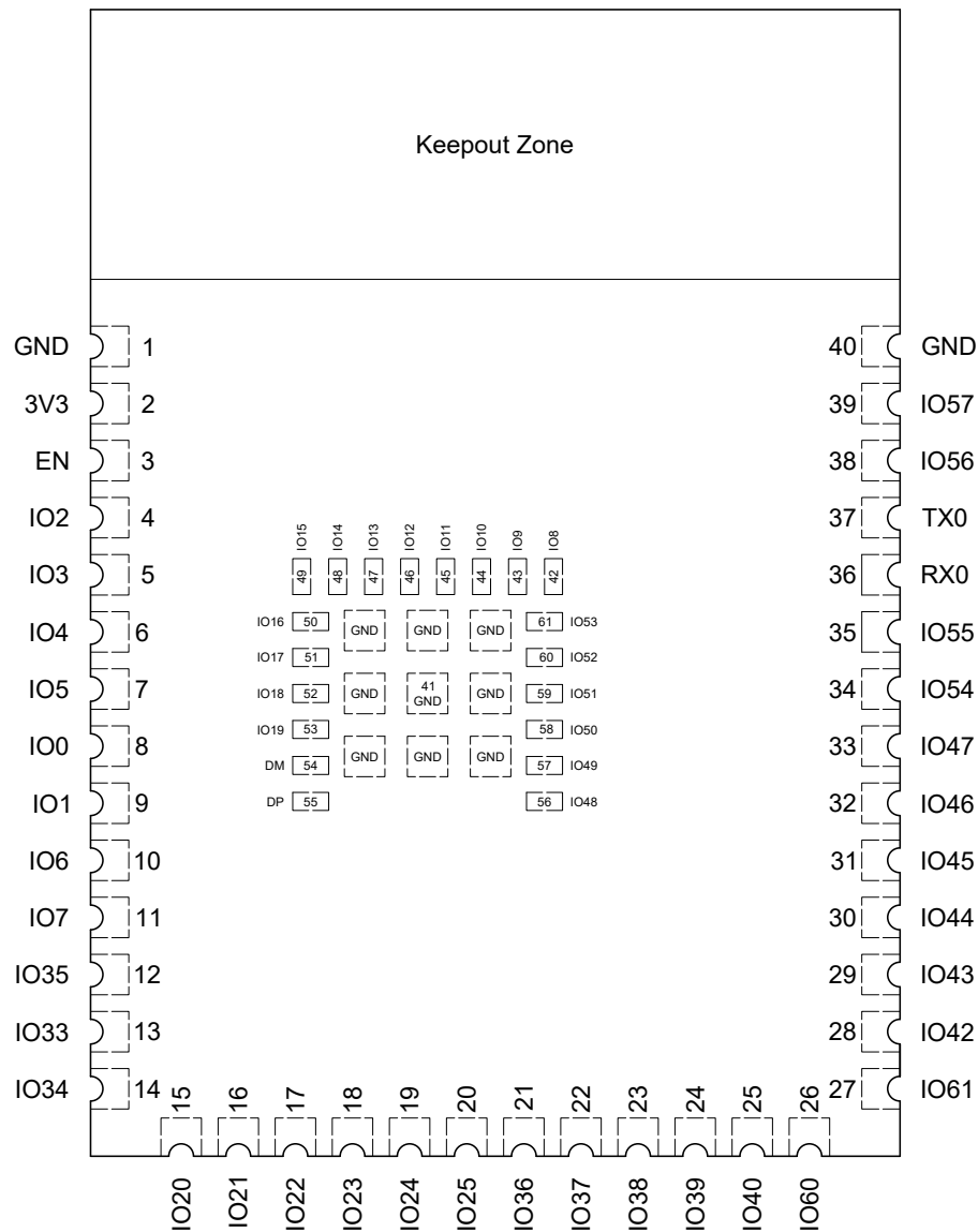
Figure 3-1. ESP32-S31-WROOM-1 Pin Layout (Top View)
