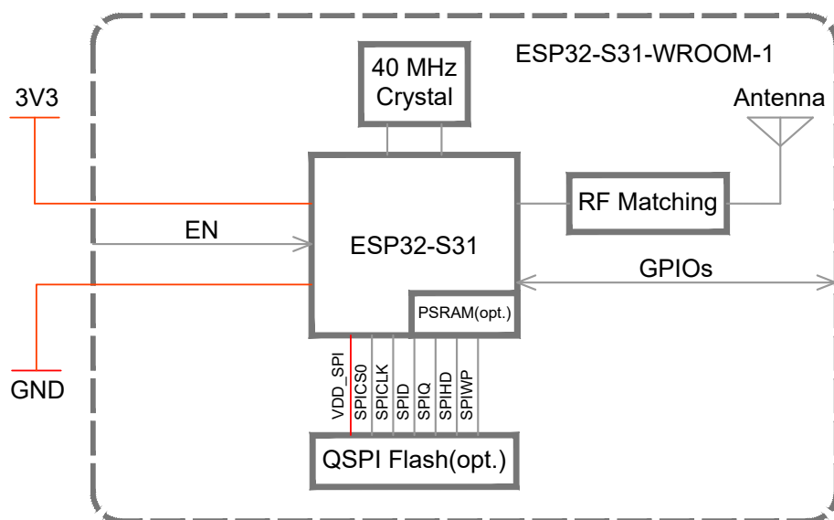
Figure 2-1. ESP32-S31-WROOM-1 Block Diagram
