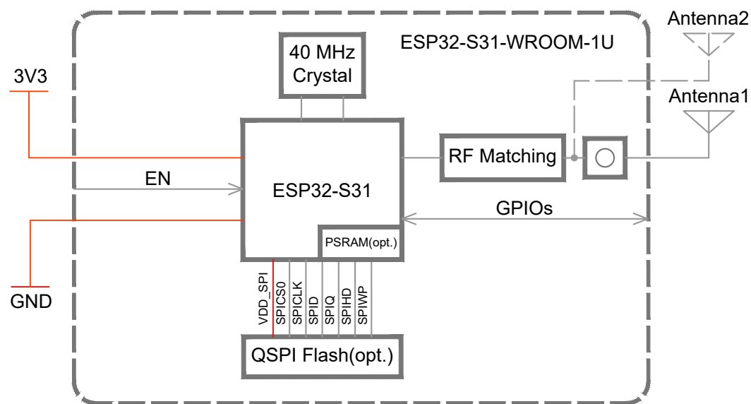
Figure 2-2. ESP32-S31-WROOM-1U Block Diagram
