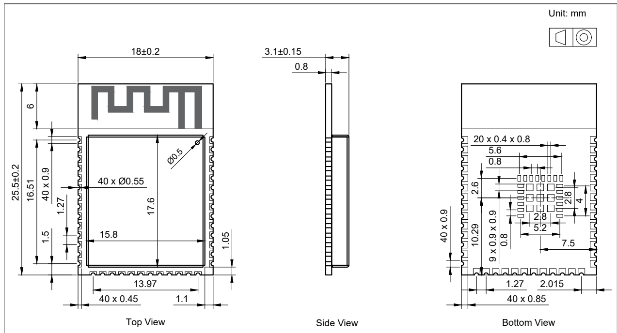
Figure 10-1. ESP32-S31-WROOM-1 Physical Dimensions
