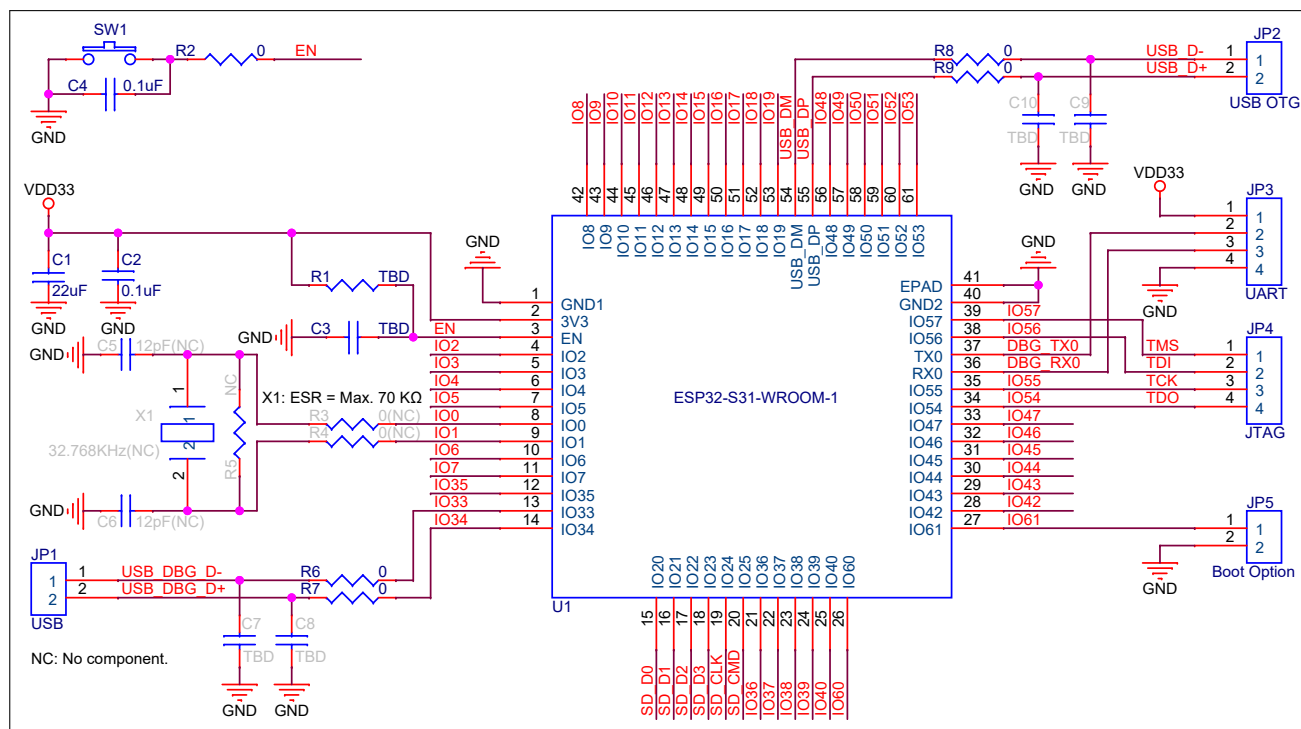
Figure 9-1. ESP32-S31-WROOM-1 Peripheral Schematics
