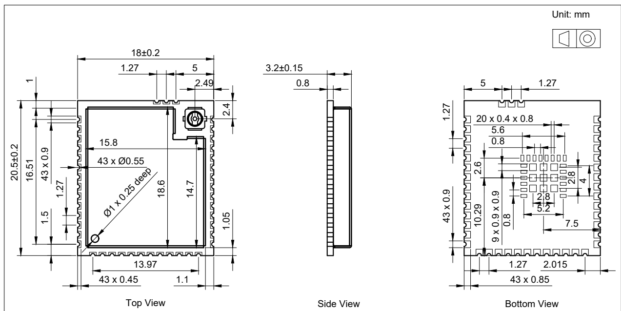
Figure 10-2. ESP32-S31-WROOM-1U Physical Dimensions
