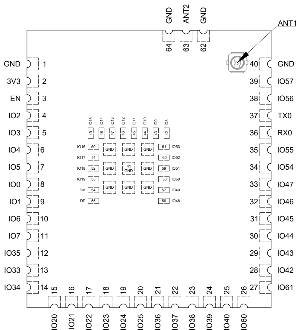
Figure 3-2. ESP32-S31-WROOM-1U Pin Layout (Top View)
