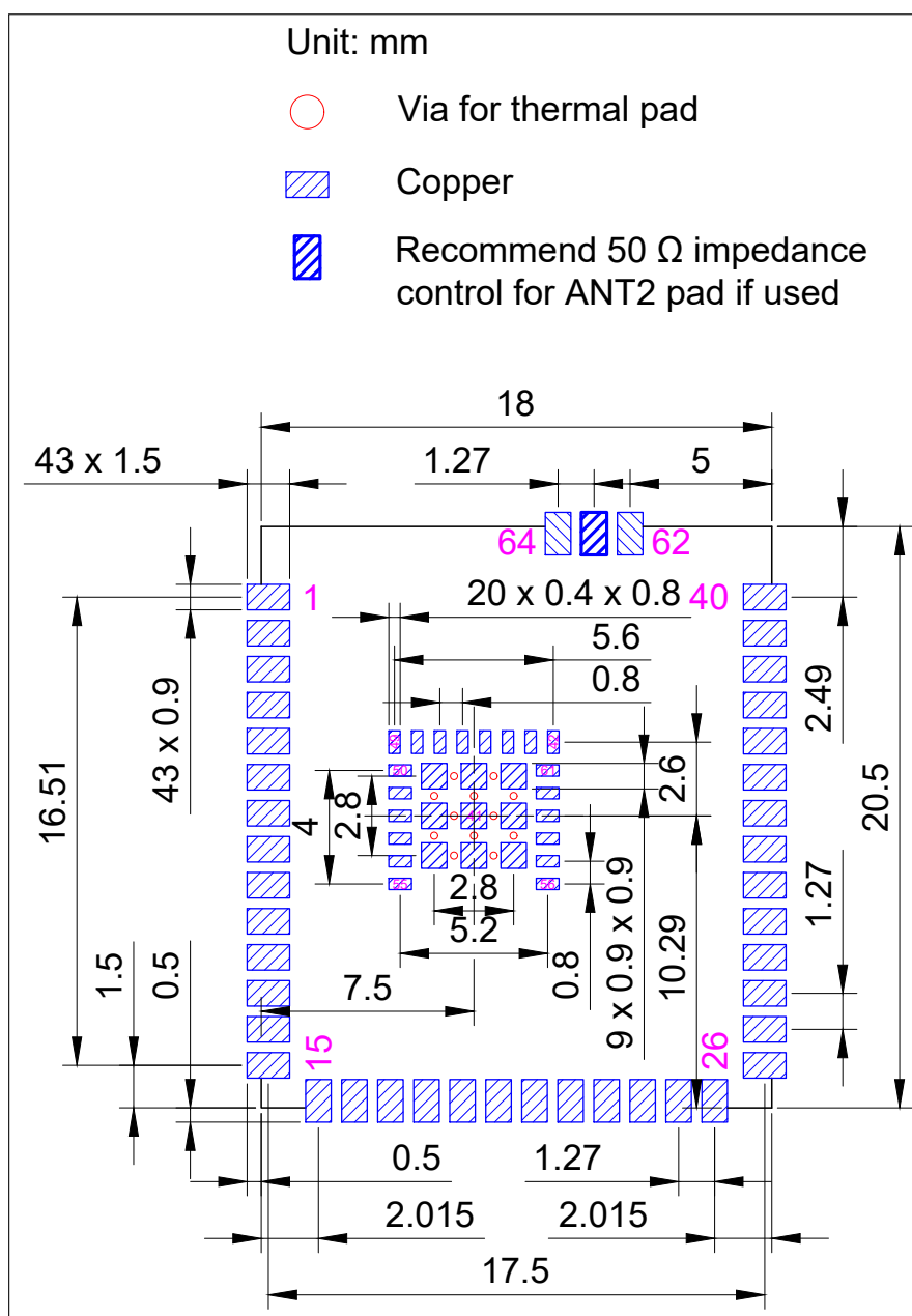
Figure 11-2. ESP32-S31-WROOM-1U Recommended PCB Land Pattern
