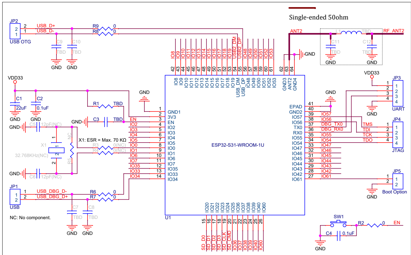
Figure 9-2. ESP32-S31-WROOM-1U Peripheral Schematics
