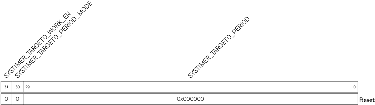
Register 10.12. SYSTIMER_TARGET0_CONF_REG (0x002C)
