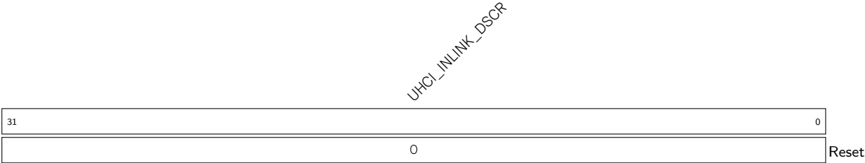
Register 23.68. UHCI_DMA_IN_DSCR_REG (0x004C)
