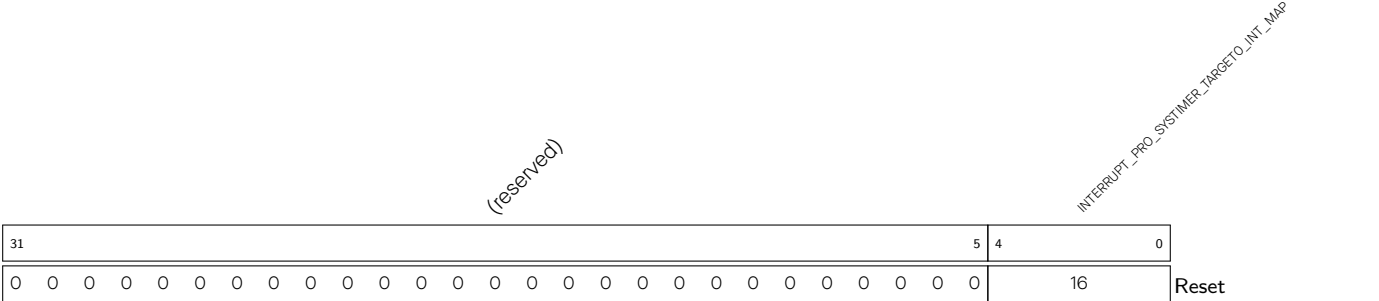
Register 8.49. INTERRUPT_PRO_SYSTIMER_TARGET0_INT_MAP_REG (0x011C)
