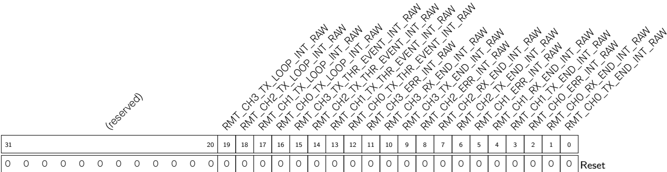
Register 31.13. RMT_INT_RAW_REG (0x0050)
