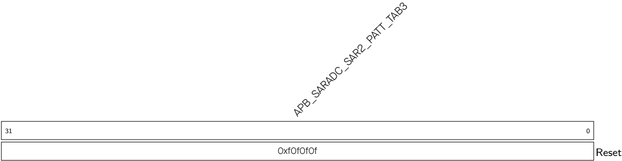
Register 32.25. APB_SARADC_SAR2_PATT_TAB3_REG (0x0030)
