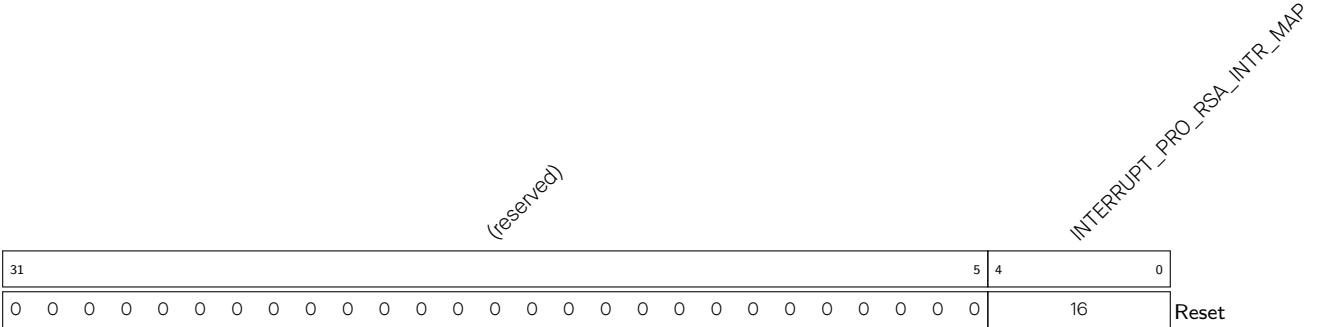
Register 8.33. INTERRUPT_PRO_RSA_INTR_MAP_REG (0x00D8)
