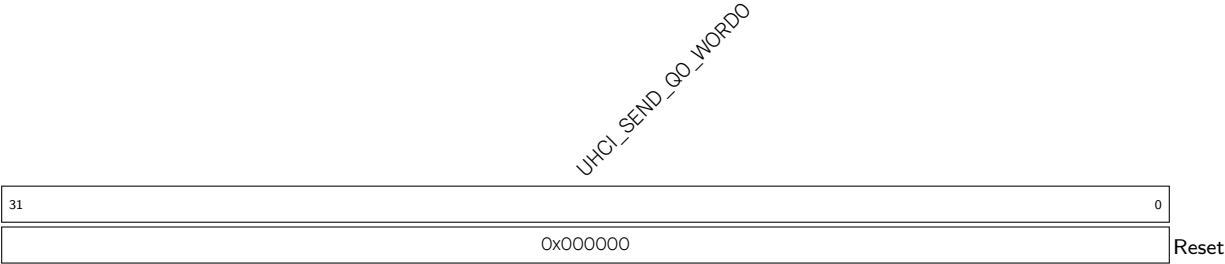
Register 23.37. UHCI_Q0_WORD0_REG (0x0078)
