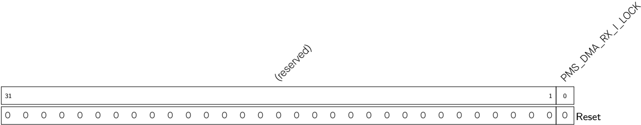
Register 14.8. PMS_DMA_RX_I_O_REG (0x009C)
