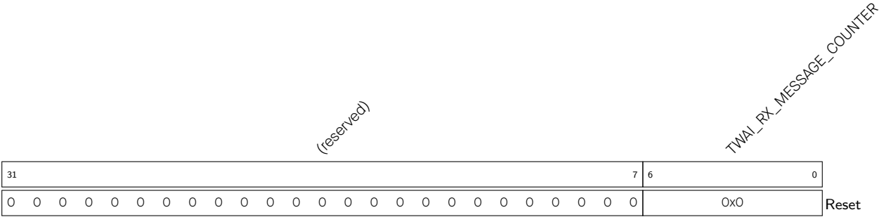
Register 29.25. TWAI_RX_MESSAGE_CNT_REG (0x0074)
