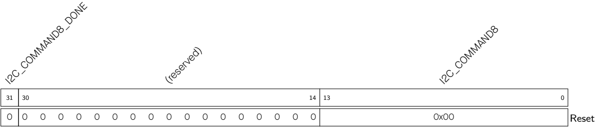
Register 25.34. I2C_COMD8_REG (0x0078)
