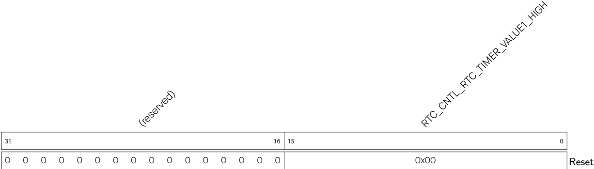
Register 9.13. RTC_CNTL_TIME_HIGH1_REG (0x00EC)
