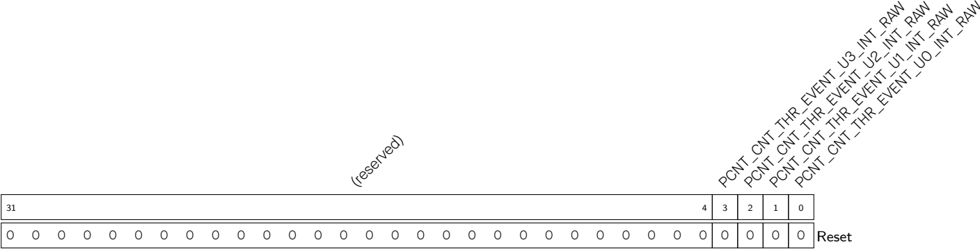
Register 27.7. PCNT_INT_RAW_REG (0x0040)
