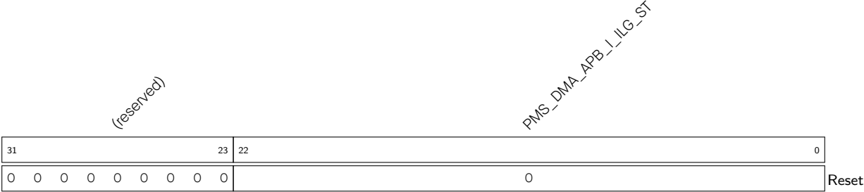
Register 14.50. PMS_DMA_APB_I_3_REG (0x0098)
