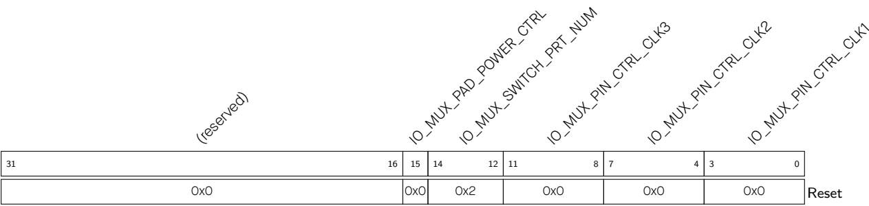
Register 5.34. IO_MUX_PIN_CTRL_REG (0x0000)
