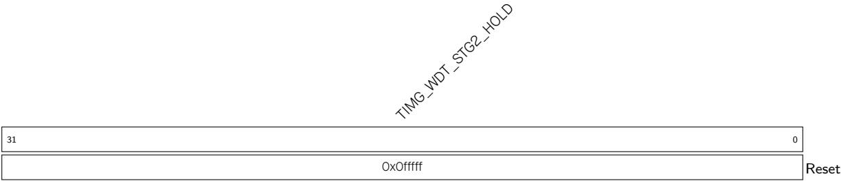
Register 11.14. TIMG_WDTCONFIG4_REG (0x0058)
