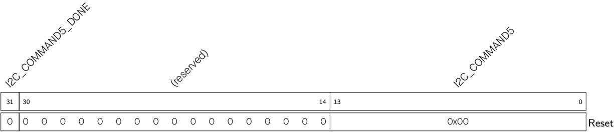
Register 25.31. I2C_COMD5_REG (0x006C)
