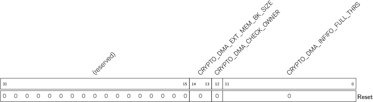
Register 2.21. CRYPTO_DMA_CONF1_REG (0x002C)
