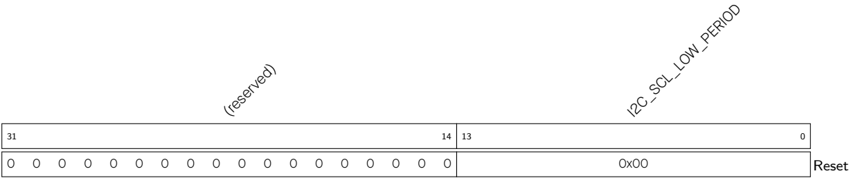
Register 25.1. I2C_SCL_LOW_PERIOD_REG (0x0000)
