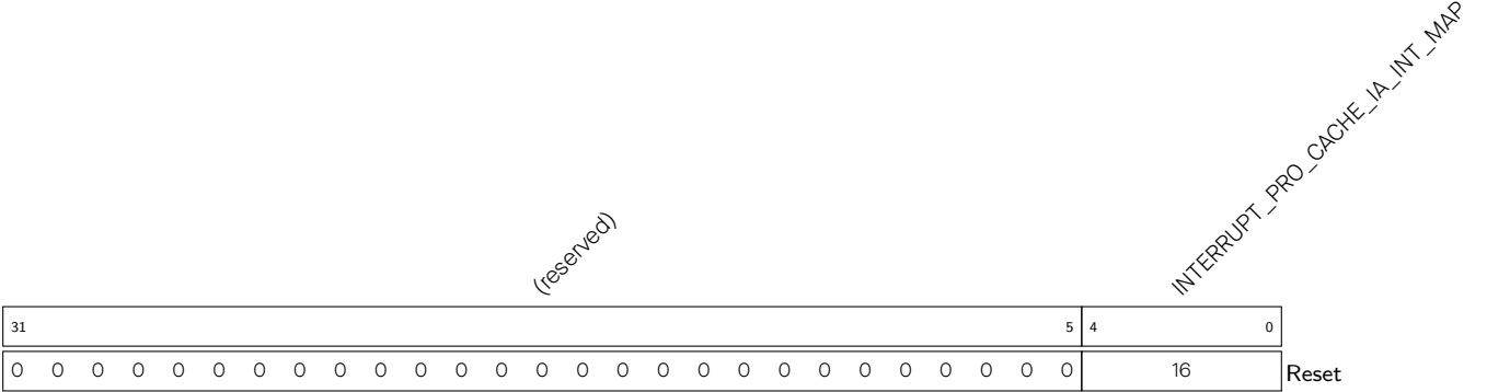
Register 8.48. INTERRUPT_PRO_CACHE_IA_INT_MAP_REG (0x0118)
