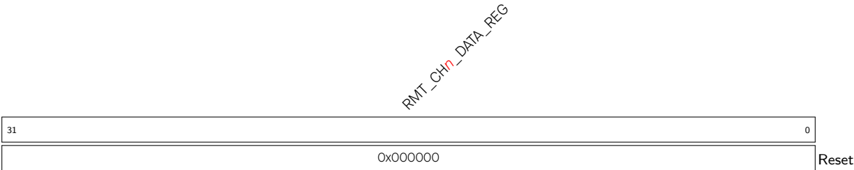
Register 31.12. RMT_CHnDATA_REG (n: 0-3) (0x0000+4*n)
