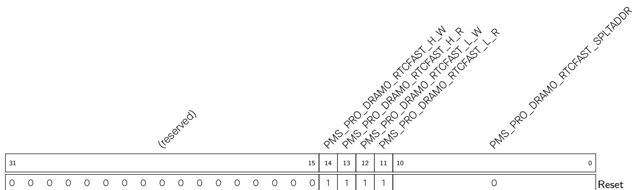
Register 14.20. PMS_PRO_DRAMO_2_REG (0x0030)
