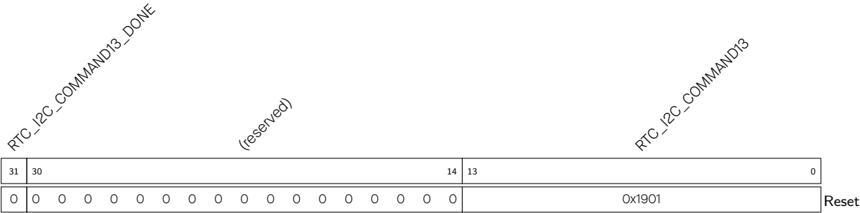
Register 1.41. RTC_I2C_CMD13_REG (0x006C)
