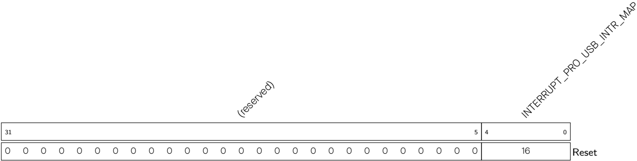
Register 8.27. INTERRUPT_PRO_USB_INTR_MAP_REG (0x00C0)
