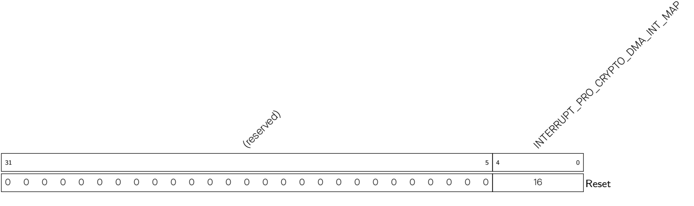
Register 8.66. INTERRUPT_PRO_CRYPTODMA_INT_MAP_REG (0x0168)
