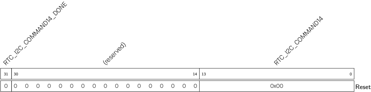
Register 1.42. RTC_I2C_CMD14_REG (0x0070)
