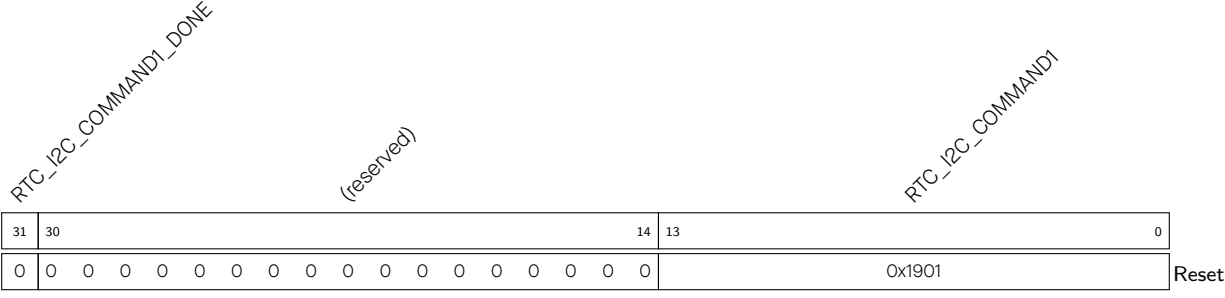
Register 1.29. RTC_I2C_CMD1_REG (0x003C)
