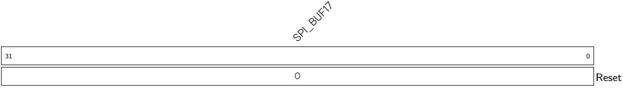
Register 24.54. SPI_W17_REG (0x00DC)
