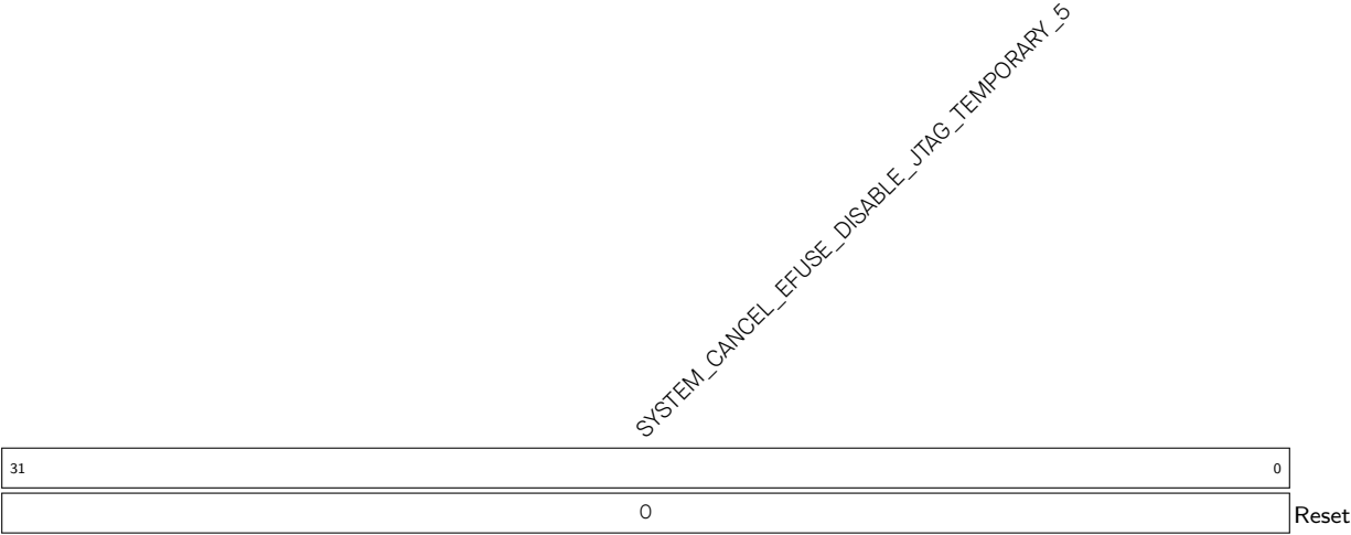
Register 15.13. SYSTEM_JTAG_CTRL_5_REG (0x0030)
