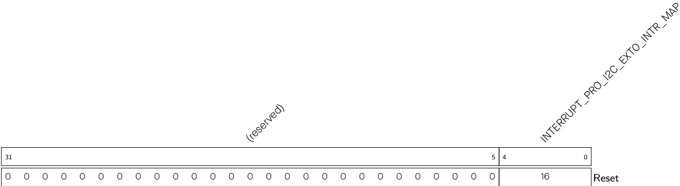
Register 8.31. INTERRUPT_PRO_I2C_EXT0_INTR_MAP_REG (0x00D0)
