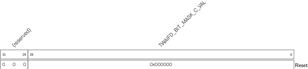
Register 38.38. TWAIFD_FILTER_C_MASK_REG (0x004C)
