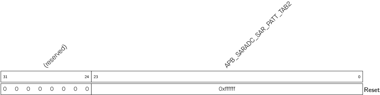
Register 46.5. APB_SARADC_SAR_PATT_TAB2_REG (0x001C)
