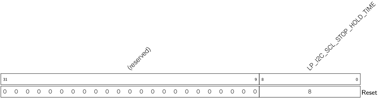
Register 34.42. LP_I2C_SCL_STOP_HOLD_REG (0x0048)
