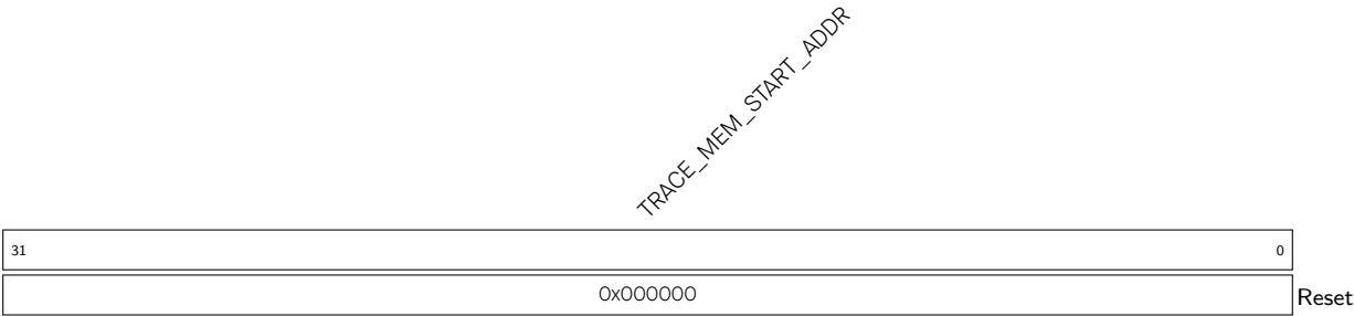
Register 3.1. TRACE_MEM_START_ADDR_REG (0x0000)
