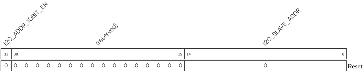
Register 34.13. I2C_SLAVE_ADDR_REG (0x0010)
