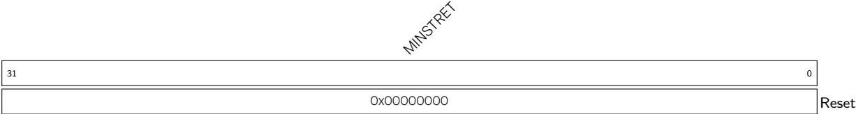
Register 2.28. minstret (0xB02)
