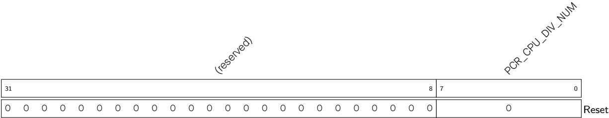
Register 9.65. PCR_CPU_FREQ_CONF_REG (0x0118)
