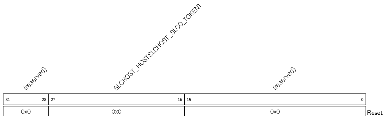
Register 39.50. SLCHOST_SLCOHST_TOKEN_RDATA_REG (0x0044)
