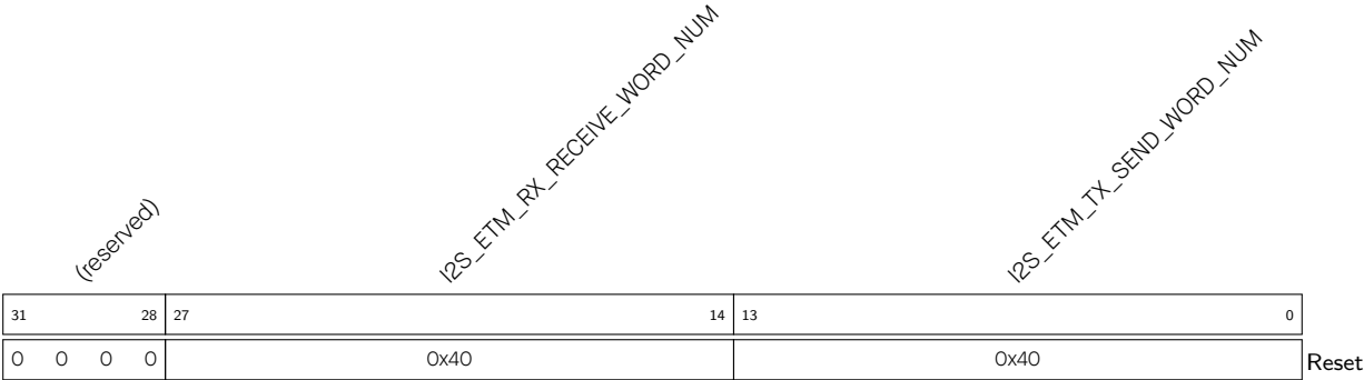
Register 35.19. I2S_ETM_CONF_REG (0x0070)
