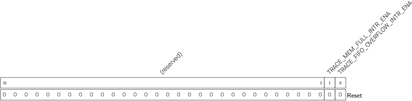
Register 3.6. TRACE_INTR_ENA_REG (0x0014)
