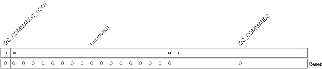
Register 34.28. I2C_COMD3_REG (0x0064)
