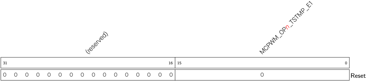
Register 41.36. MCPWM_OPn_TSTMP_E1_REG (n: 0-2) (0x012C+0x8*n)
