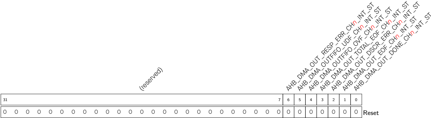
Register 5.6. AHB_DMA_OUT_INT_ST_CHn_REG (n: 0-2) (0x0034+0x10*n)
