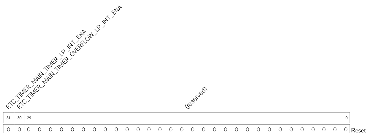
Register 17.16. RTC_TIMER_LP_INT_ENA_REG (0x0040)
