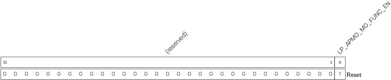
Register 18.49. LP_APMO_FUNC_CTRL_REG (0x00C4)
