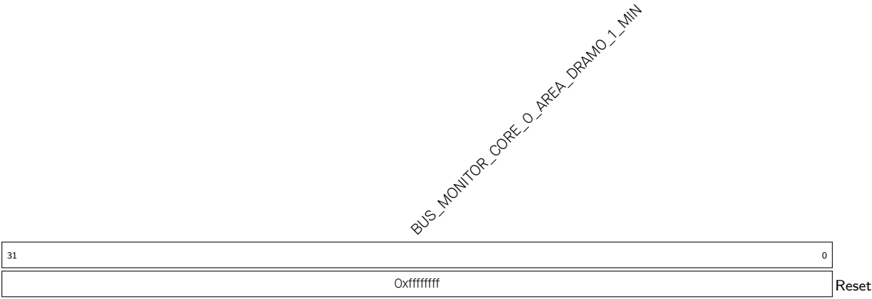
Register 20.19. BUS_MONITOR_CORE_0_AREA_DRAMO_1_MIN_REG (0x0018)
