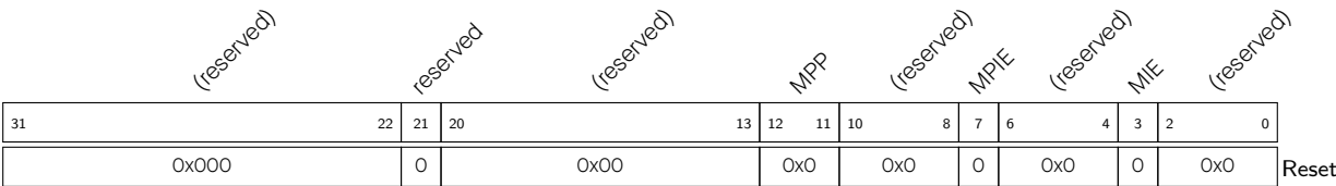
Register 4.2. mstatus (0x300)
