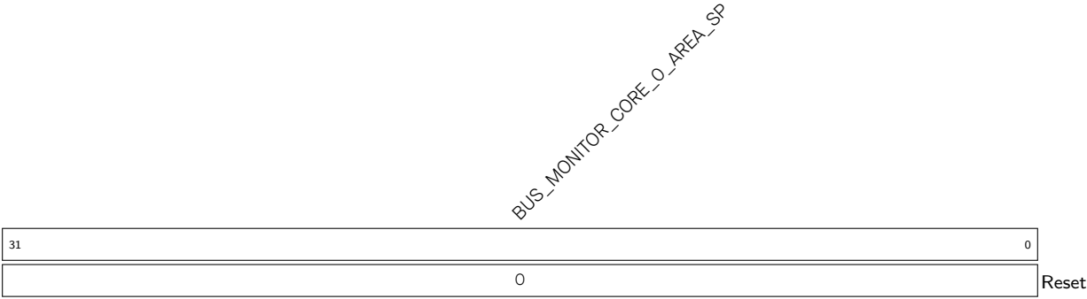
Register 20.26. BUS_MONITOR_CORE_0_AREA_SP_REG (0x0034)
