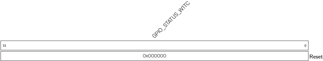
Register 8.13. GPIO_STATUS_W1TC_REG (0x007C)
