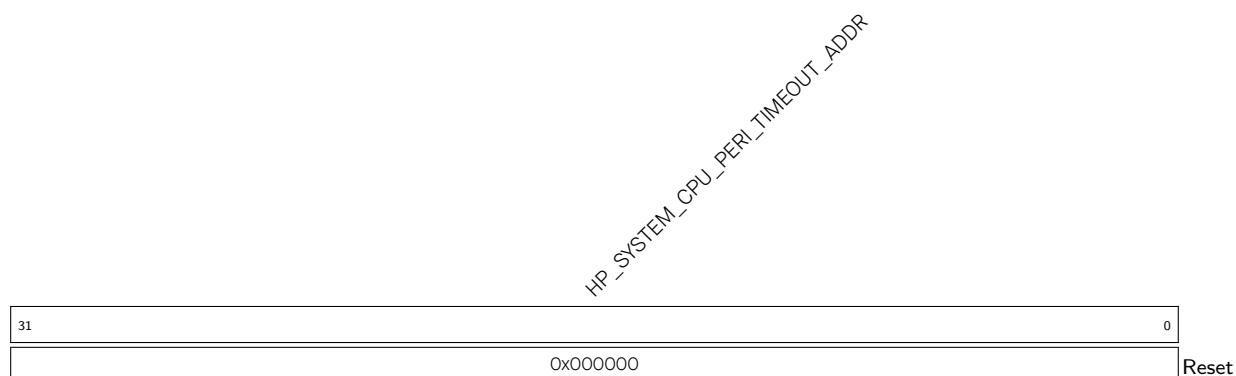
Register 19.6. HP_SYSTEM_CPU_PERI_TIMEOUT_ADDR_REG (0x0010)
