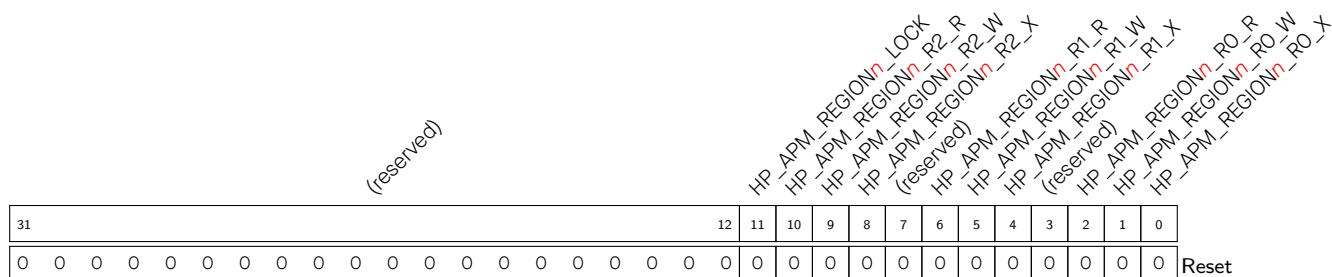
Register 18.4. HP_APM_REGION n _ATTR_REG ( n : 0-15) (0x000C+0xC* n )
