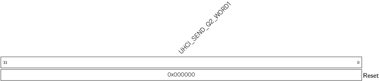
Register 26.45. UHCI_REG_Q2_WORD1_REG (0x0048)
