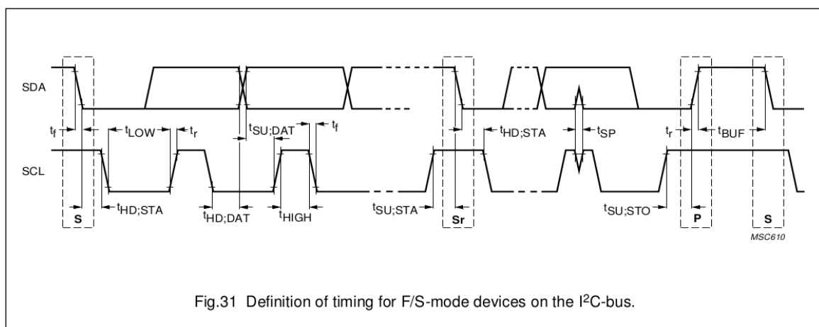
图 28.3-3. I2C 协议时序 (引自 The I2C-bus specification Version 2.1 Fig.31)
