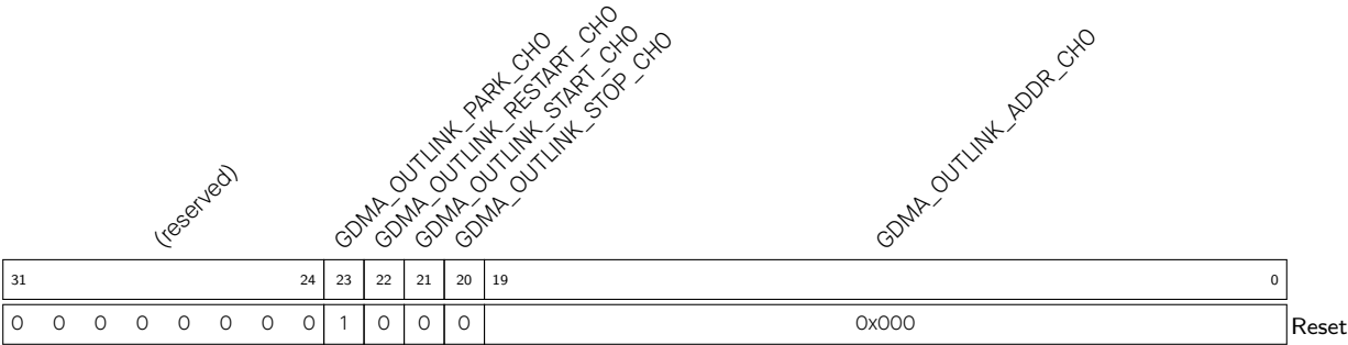
Register 2.14. GDMA_OUT_LINK_CH n _REG ( n : 0-2) (0x00E0+192* n )
