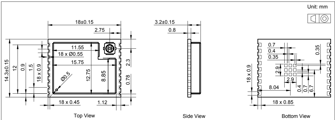
Figure 10-2. ESP32-C3-WROOM-02U Physical Dimensions
