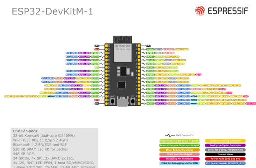
Fig. 3: ESP32-DevKitM-1 (click to enlarge)
