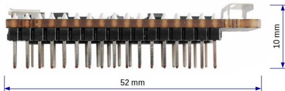
Fig. 37: ESP32-PICO-KIT dimensions - side (with male headers)
