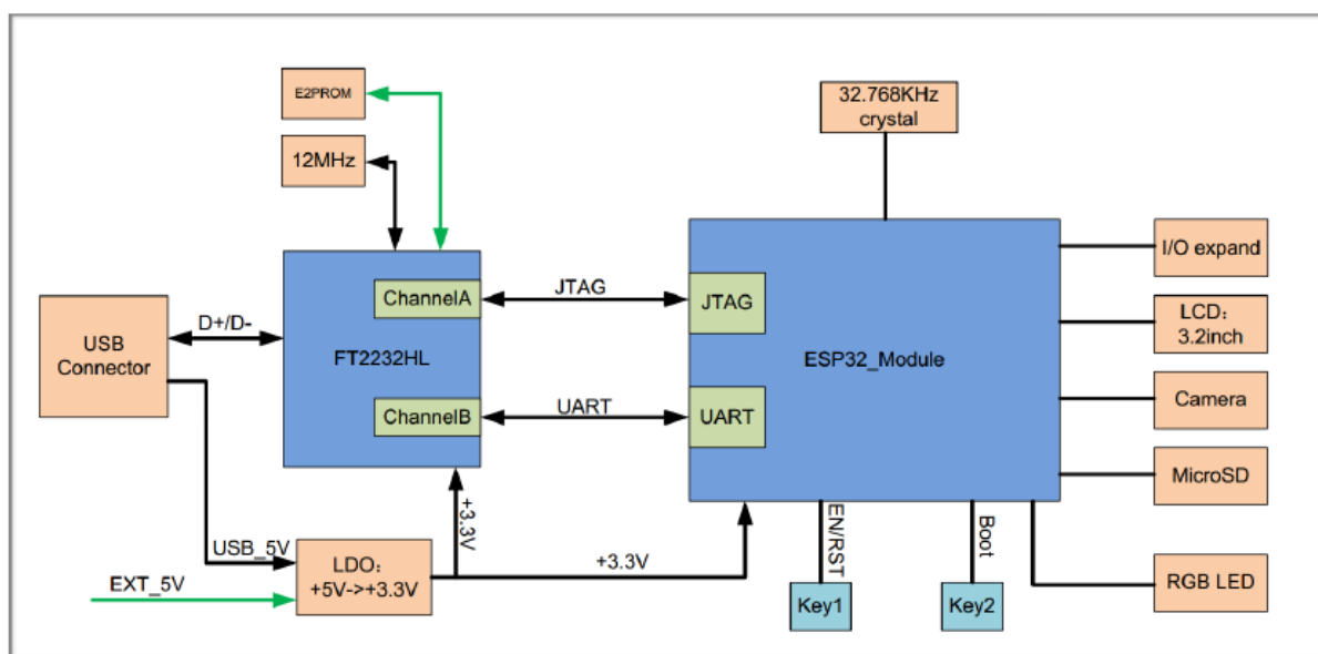
Fig. 23: ESP-WROVER-KIT block diagram
